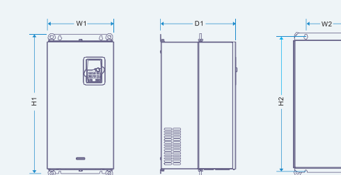
132-200kW Flange mounting Installation diagram
