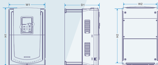
18.5-55kW Installation
