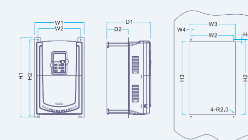
37-110kW Flange mounting Installation diagram
