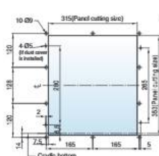
<Mounting hole>
