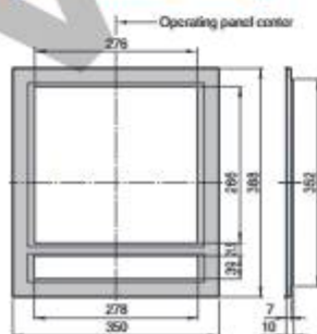
<External size>
