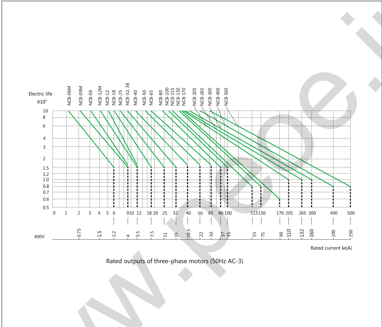
Electric life curves (AC-3 Ue=400V)
